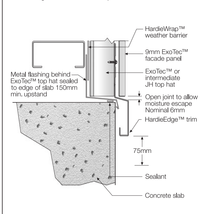
FIGURE 26B WALL BASE TYPICAL DETAIL 2 WITH HARDIEEDGE™ TRIM
