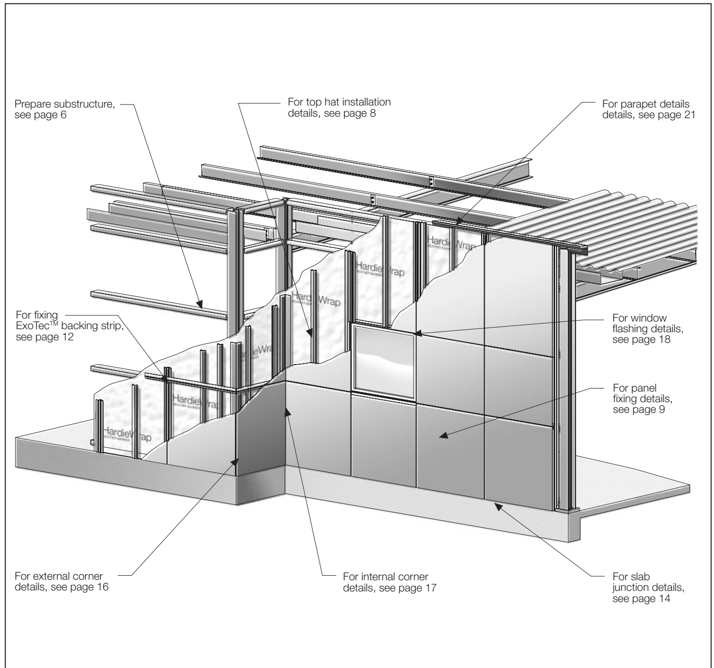
FIGURE 1 INSTALLATION OVERVIEW
